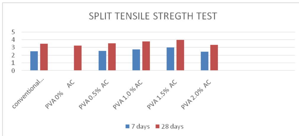
Figure 1 Graphical representation for Split tensile strength test results
